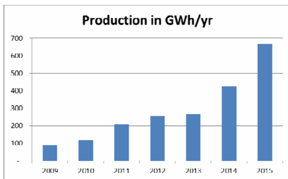
Figure 4: Combined production levels of Dutch deep geothermal doublets in GWh.
